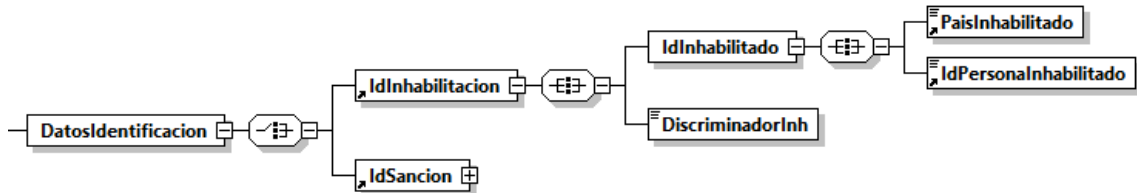
Figura 7. IdInhabilitacion
